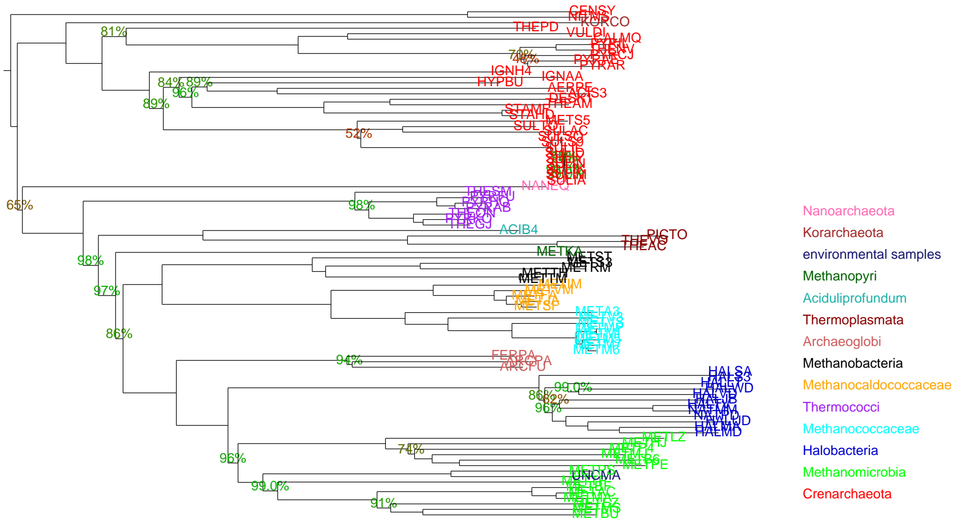
BestDimless Tree of 93 Archaea, (C) 2011 CBRG, ETH Zurich
