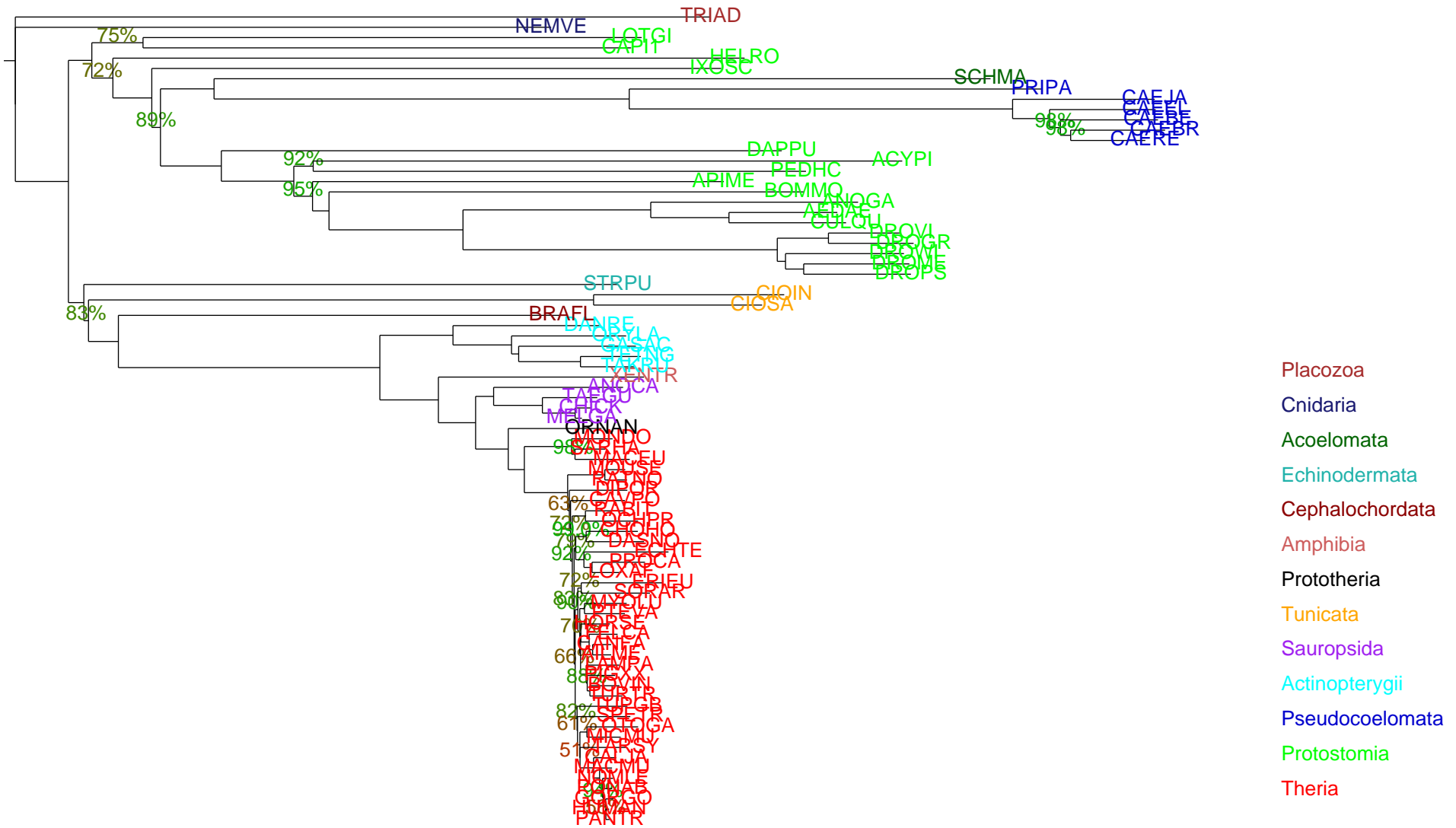
BestDimless Tree of 79 Metazoa, (C) 2012 CBRG, ETH Zurich
