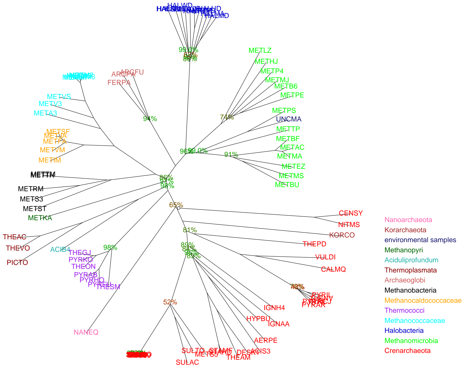
BestDimless Tree of 93 Archaea, (C) 2011 CBRG, ETH Zurich
