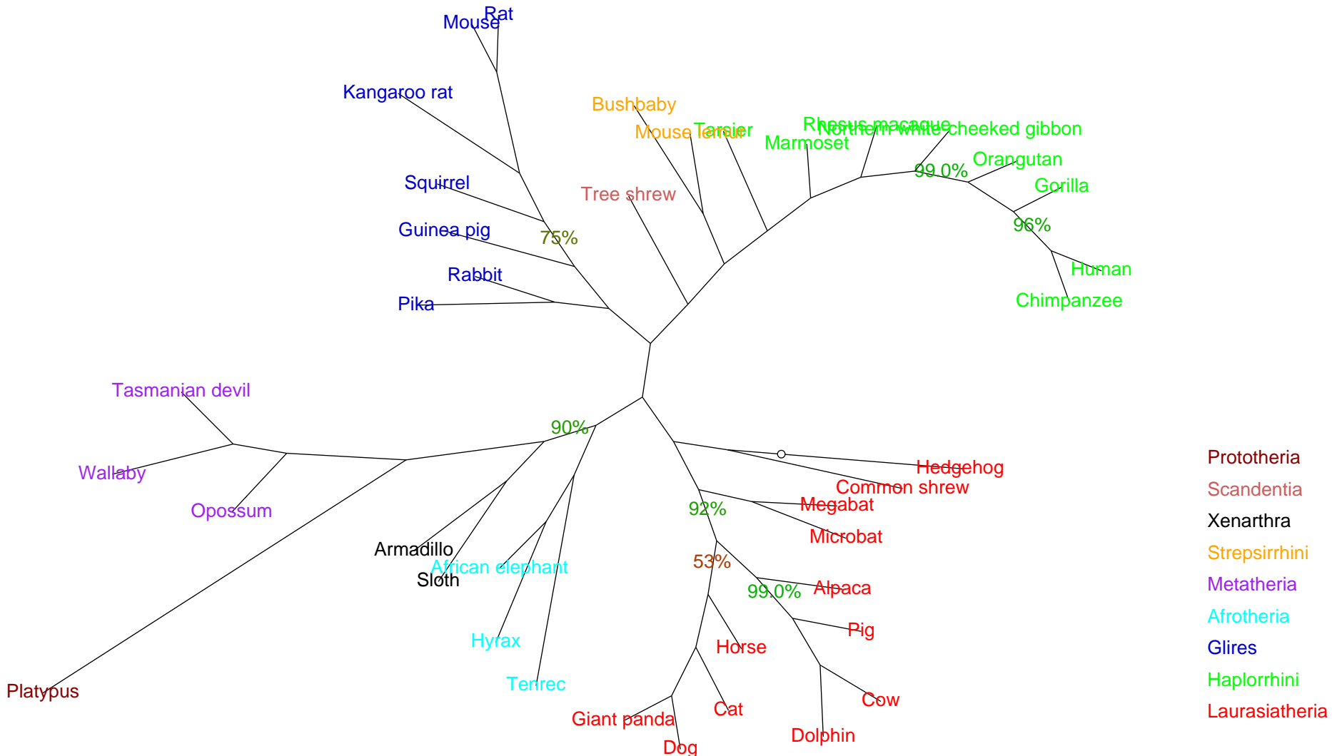
BestDimless Tree of 39 Mammalia, (C) 2012 CBRG, ETH Zurich
