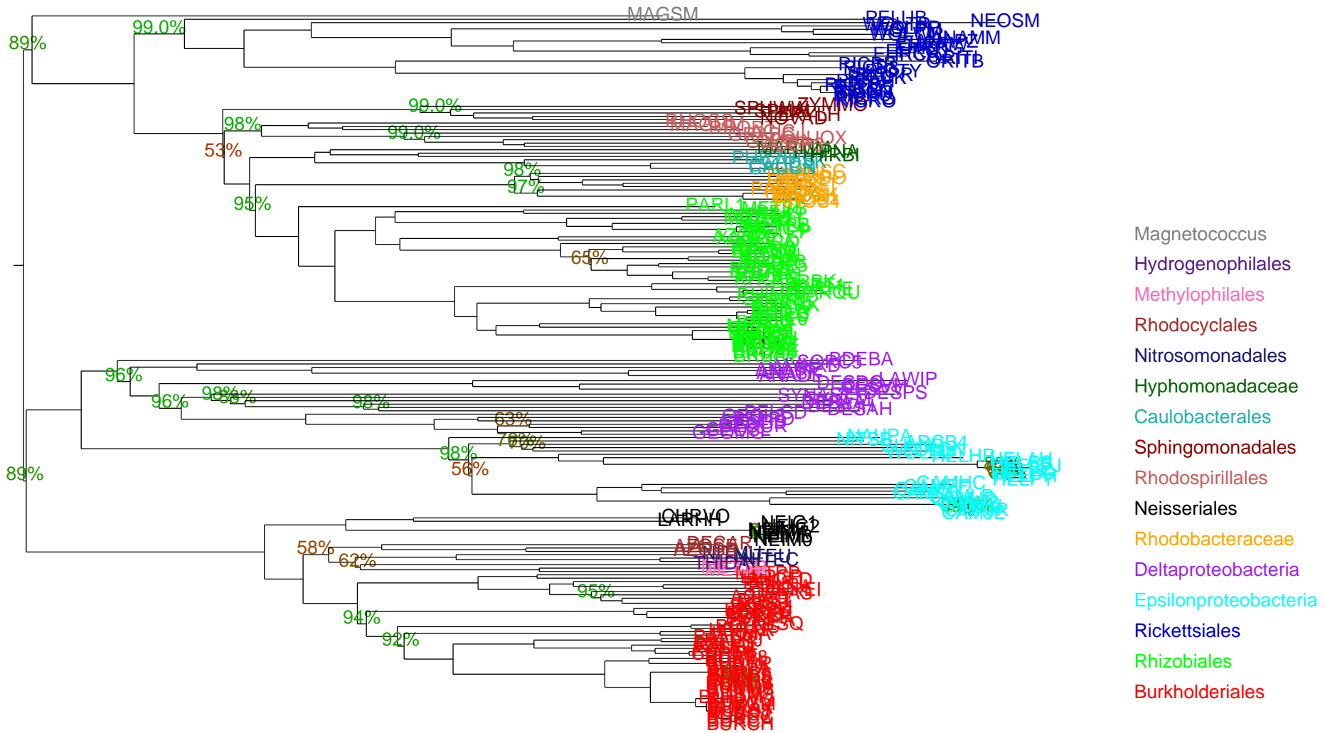
BestDimless Tree of 213 other Proteobacteria, (C) 2010 CBRG, ETH Zurich
