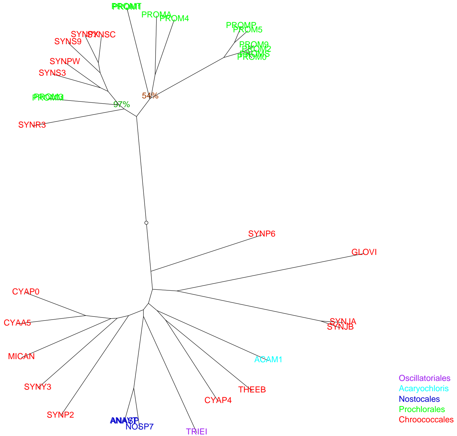
BestDimless Tree of 34 Cyanobacteria, (C) 2009 CBRG, ETH Zurich
