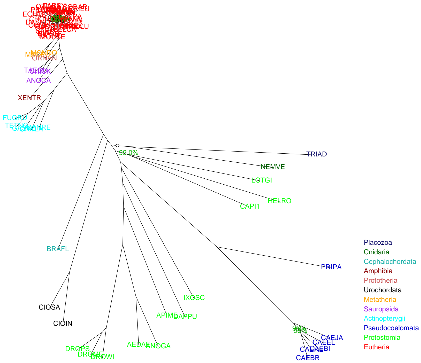
BestDimless Tree of 67 Metazoa, (C) 2010 CBRG, ETH Zurich
